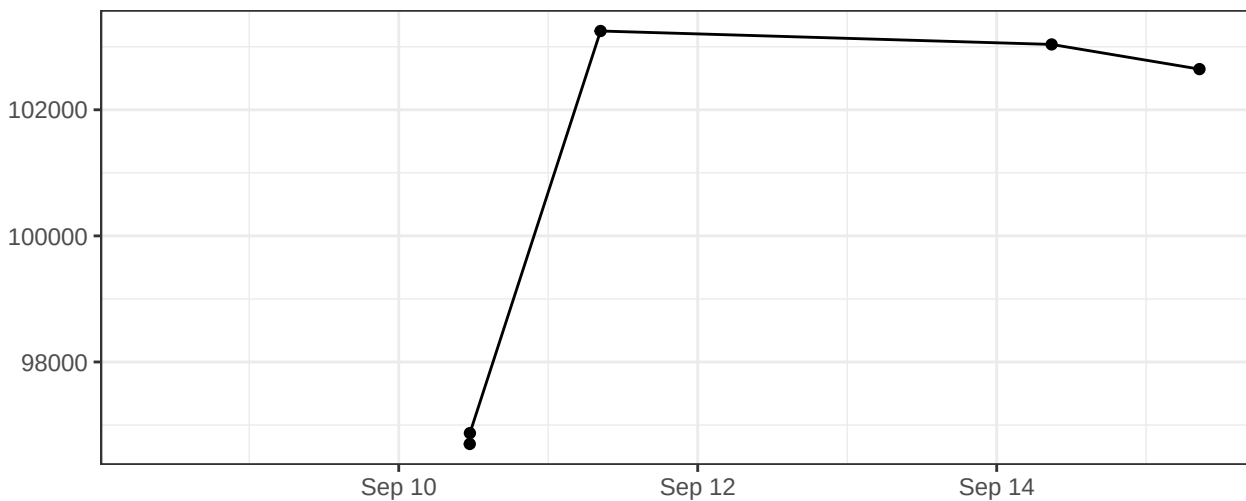
UV379-A_Gain
