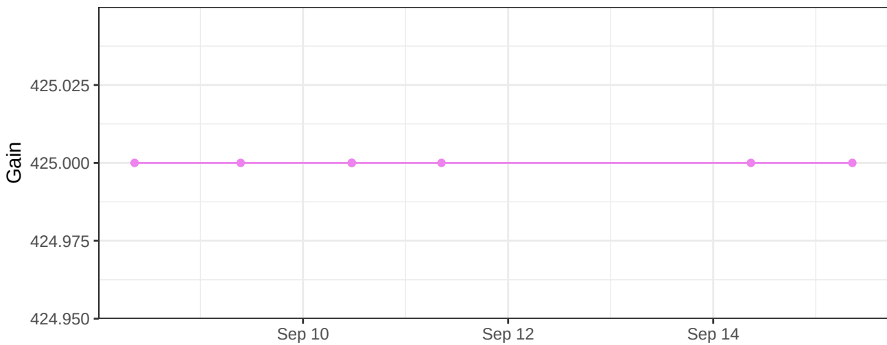
V610-A_Gain
