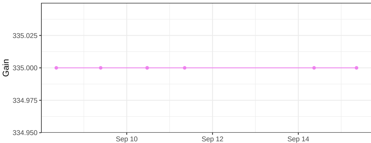
V510-A_Gain
