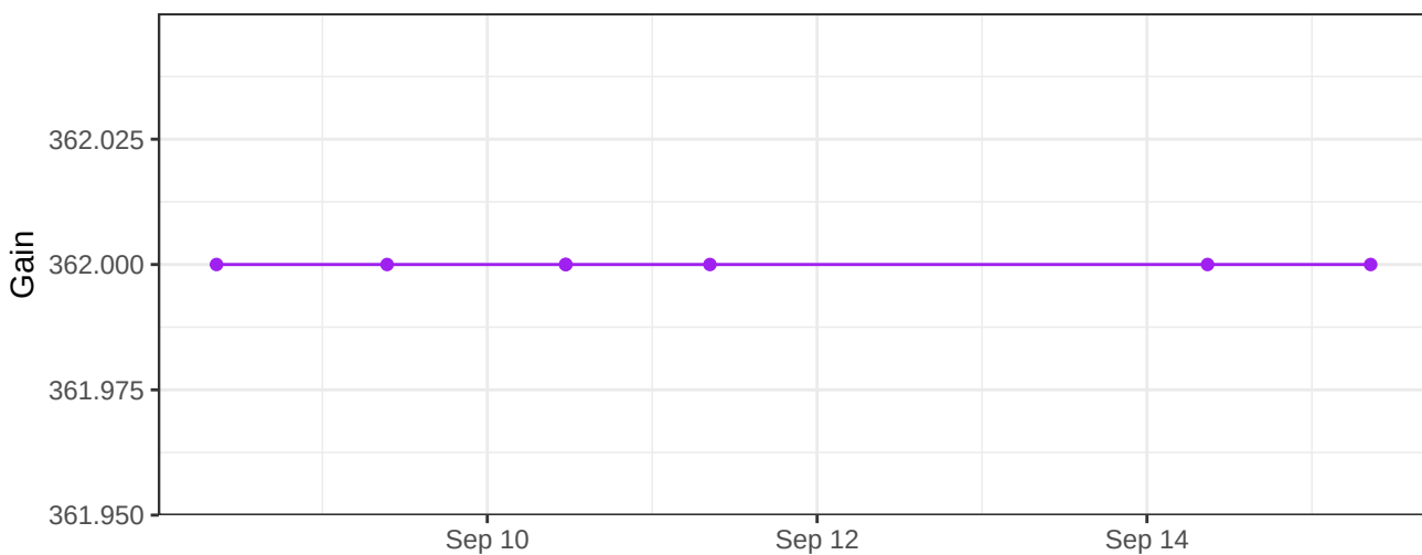
UV446-A_Gain
