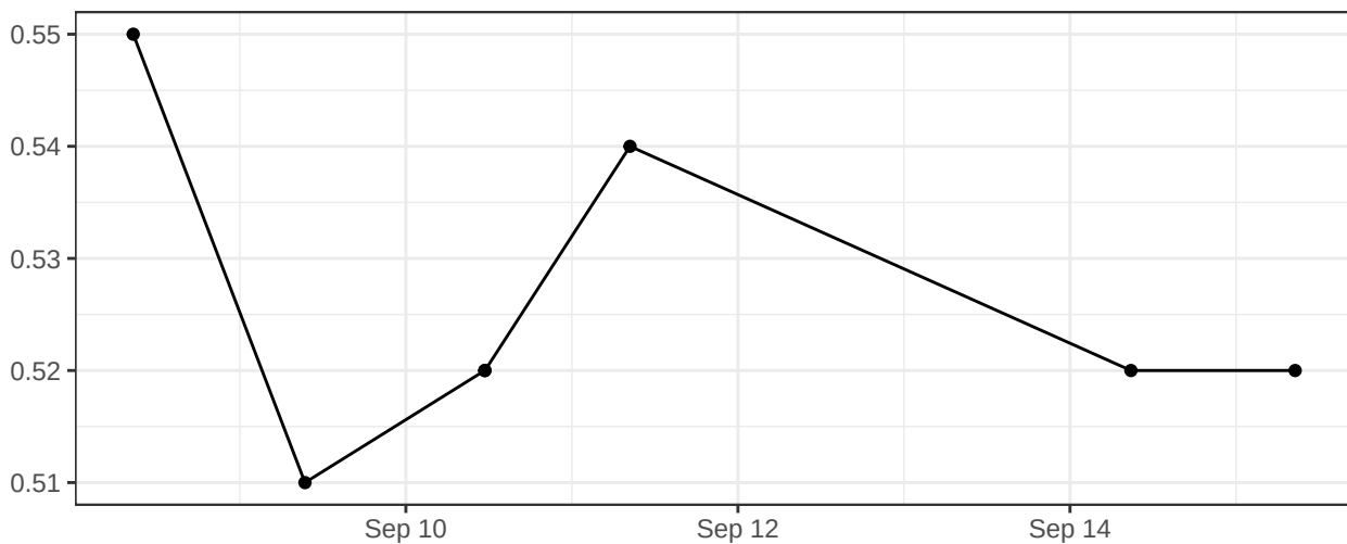
Yellgrn_AreaScalingFactor
